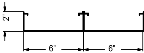
6" X 2" .062 EXTRUDED "FLUSH DECK"
