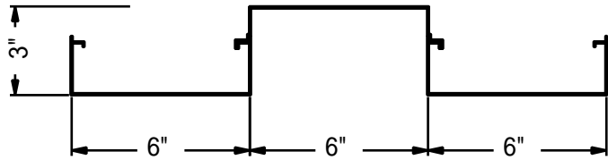
6" X 3" .062 EXTRUDED "ECONO DECK"
