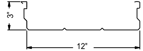
12" X 3" ROLLFORMED FLAT PAN
