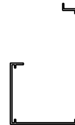
7" X 4" X .094 EXTRUDED ALUMINUM FASCIA/GUTTER
