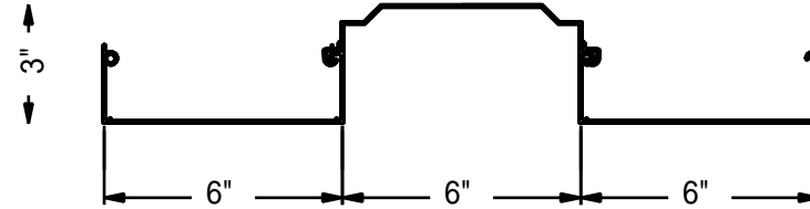
6" X 3" .075 EXTRUDED "LONG SPAN DECK"
