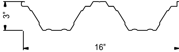
16" X 3" ROLLFORMED W-PAN
