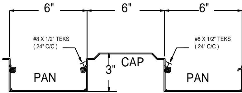
6" X 3" .075 EXTRUDED ALUMINUM "LONG SPAN DECK"
