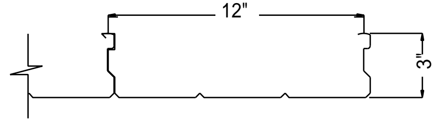
ROLLFORMED ALUMINUM FLATPAN
