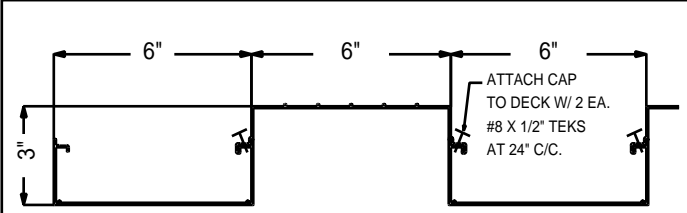
DECK ASSEMBLY ( EXTRUDED ALUMINUM ECONO DECK )
