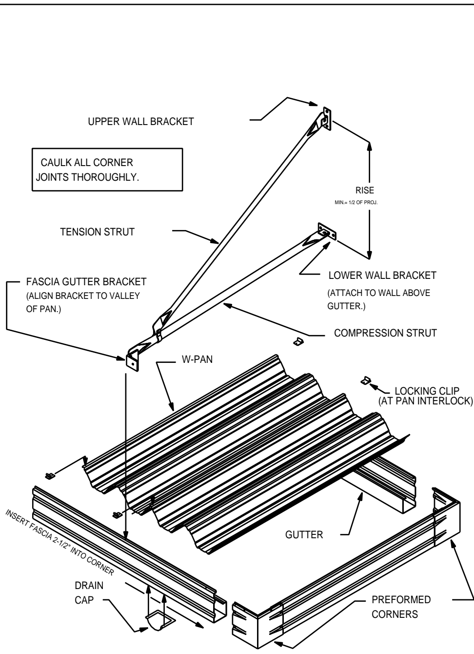
STANDARD OVERHEAD SUPPORT
