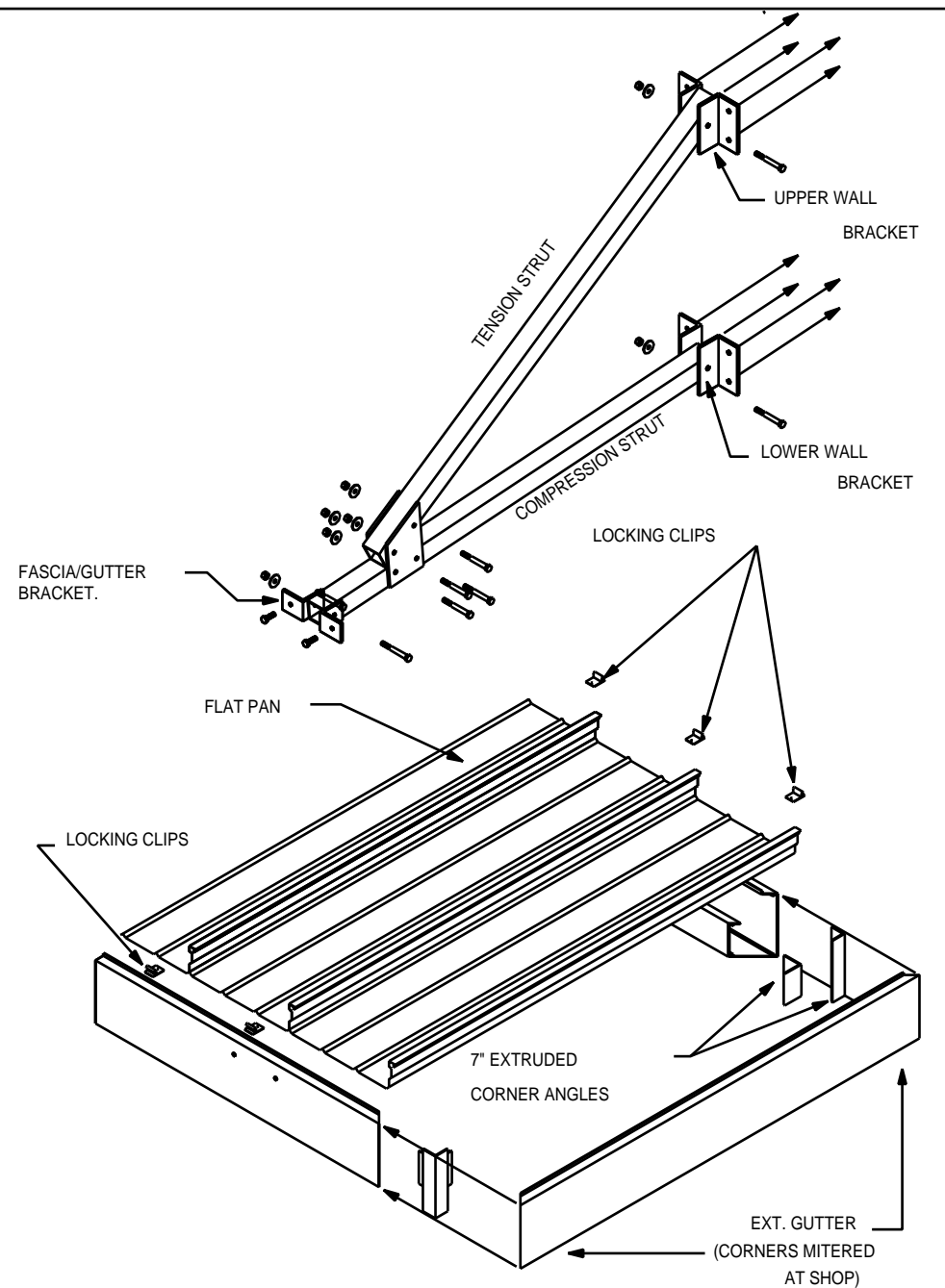
HEAVY-DUTY OVERHEAD SUPPORT
